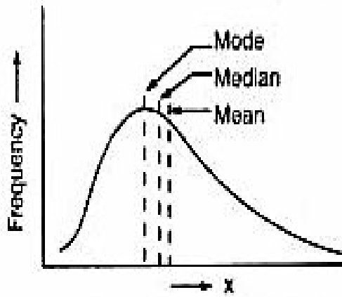
(b) Positively skewed distribution
